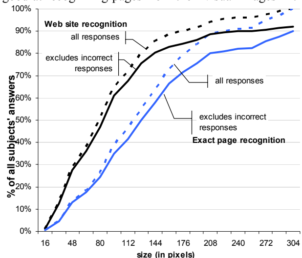
Figure 4. Running sums of thumbnail stop sizes
