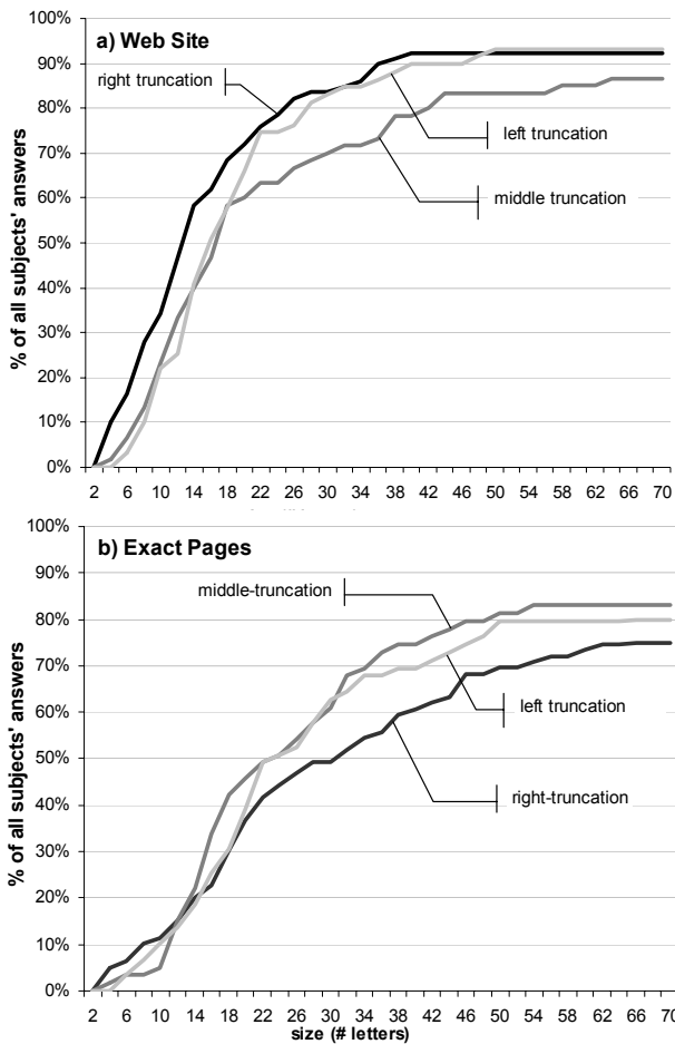
Figure 5. Running sums of title stop sizes.
