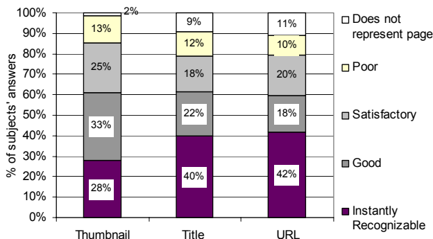
Figure 8. Subjects' ratings of thumbnails, titles and URLs
