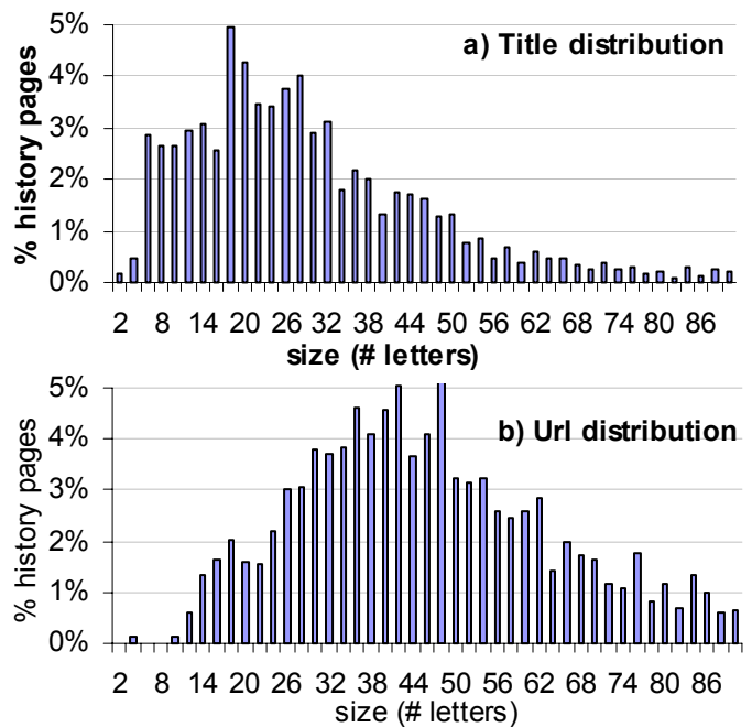
Figure 7. Distribution of title and URL lengths. responses for the three different title and URL truncation methods into ‘Titles’ and ‘URLs’ categories.
